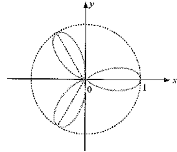
r = \cos 3\varphi (3 yapraklı gül)
